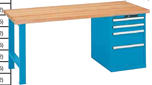
Drawer cabinet (Selection 75): 4 drawers (full extension) Heights: 2 x 100 mm, 200 mm, 300 mm
